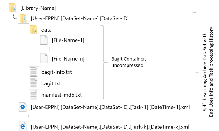
Figure 6. Archive Directory and File Structure
